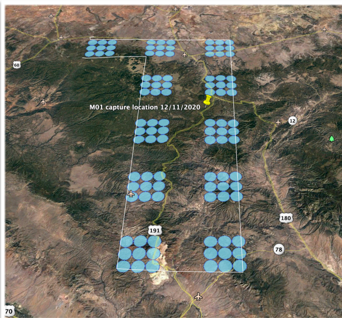
Figure 2. Spatially explicit models generate camera placement centroids by computer to capture marked (collared) or unmarked mountain lions to obtain occurrence/density data, and when combined with GPS movement, statistically valid estimates of population sizes.
