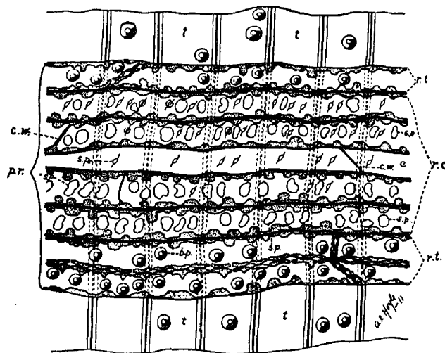
FIG. 10.—An ordinary pith ray cut longitudinally (radial section), magnified 250 diameters; p. r., pith rays; r. t., ray tracheids; r. c., ray cells; t. c. w., thin-walled ray cells; b. p., bordered pits; s. p., simple pits; t., tracheids.
